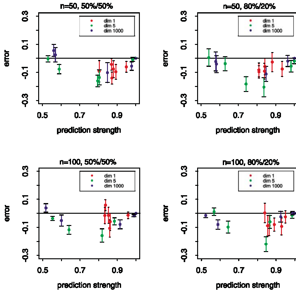
Figure 5. Bias in prediction strength estimates, for the experiments described in the text. The left panel shows the error ps_{n/2, n/2} - ps_{n, \infty} plotted as a function of the “true” prediction strength ps_{n, \infty} . The right panel assesses five-fold cross-validation, and hence ps_{4n/5, n/5} - ps_{n, \infty} is shown.
